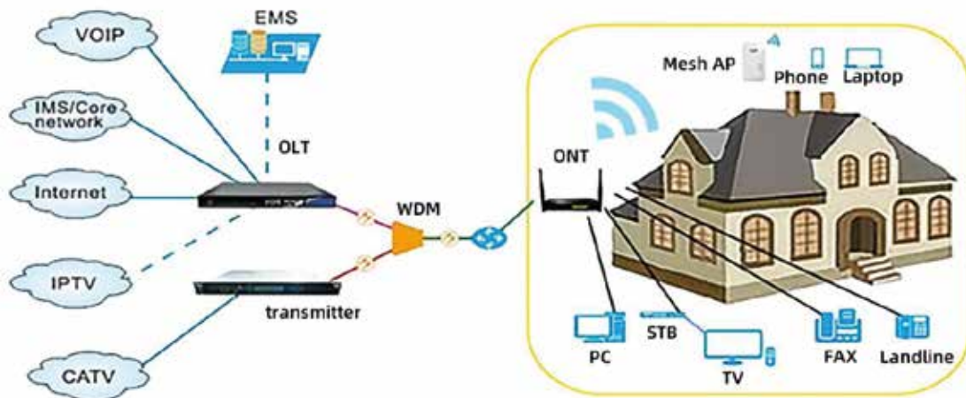
Picture 1-1 FD8411GWVC-G products Network diagram
